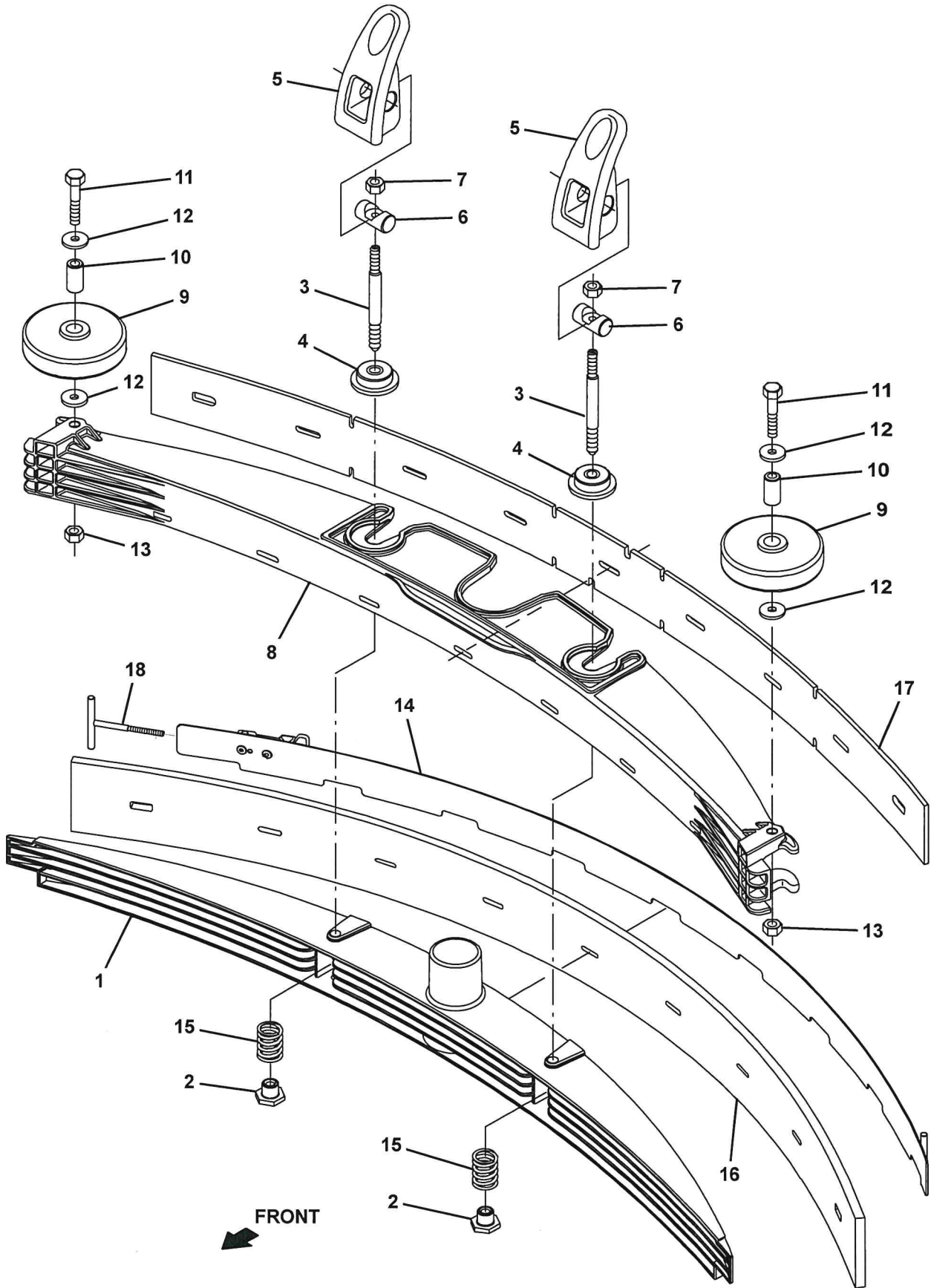
Fig. 20 – Rear Squeegee Group
