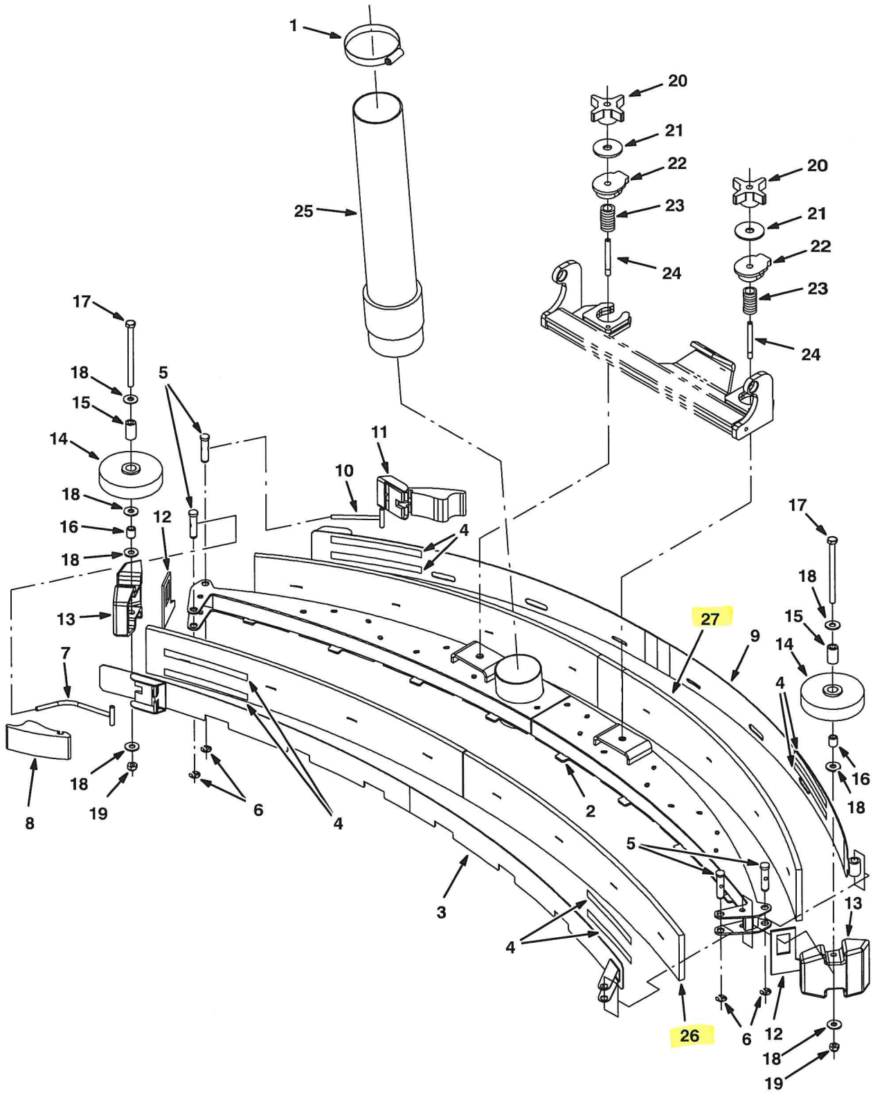
Fig. 32 - Squeegee Group, Rear
