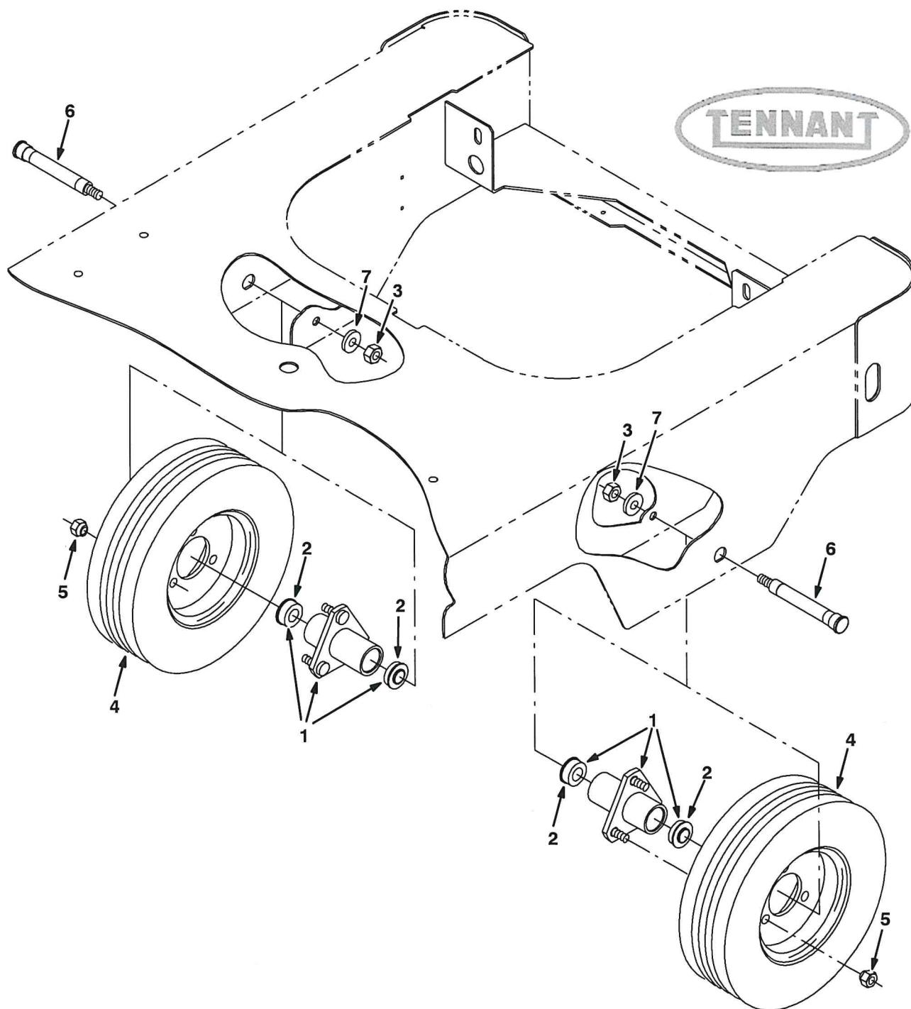
Fig. 10 - Rear Wheel Group
