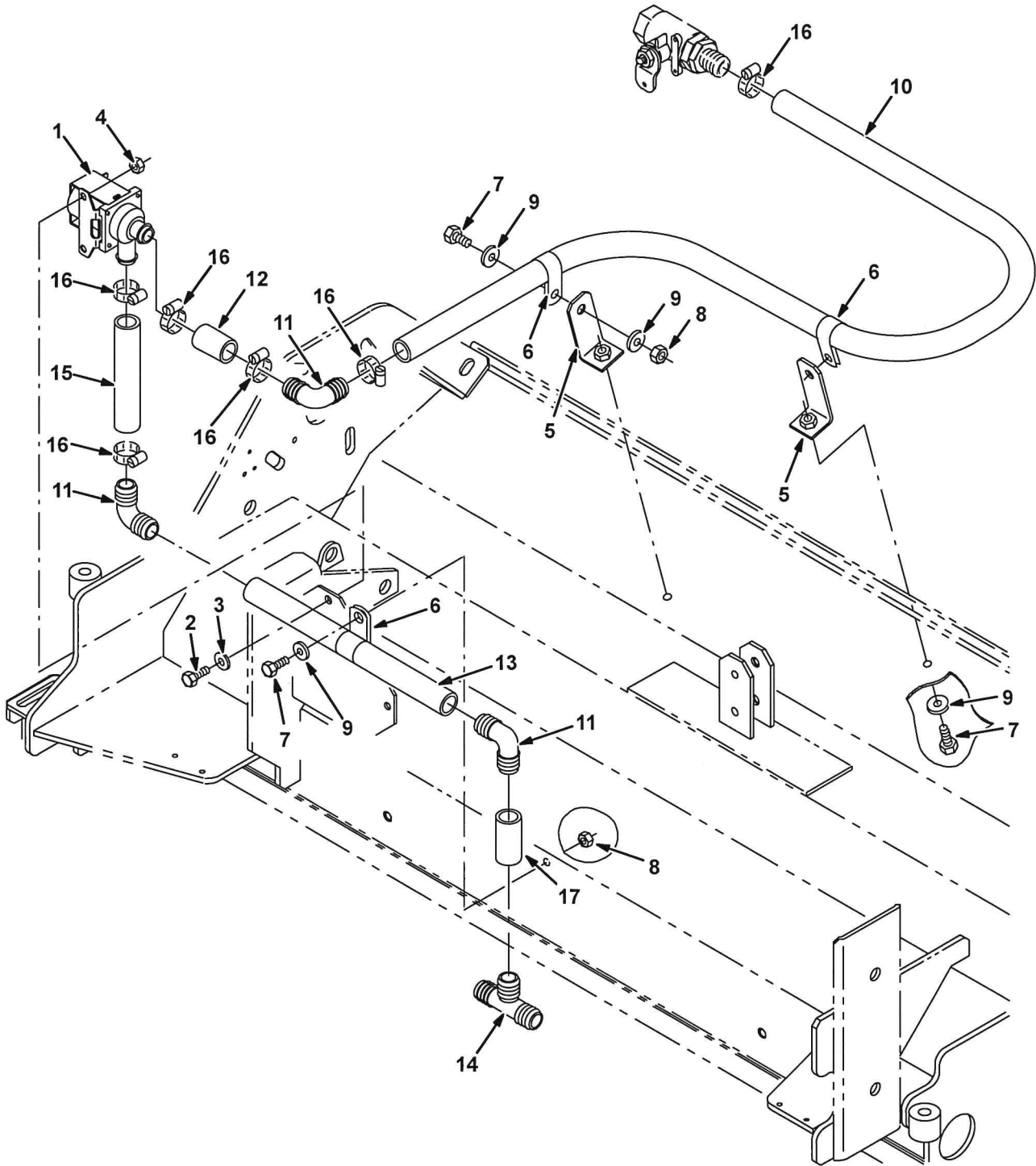
Fig. 37 – Max Pro 1200 (Cylindrical Brush) Solution Valve Group
