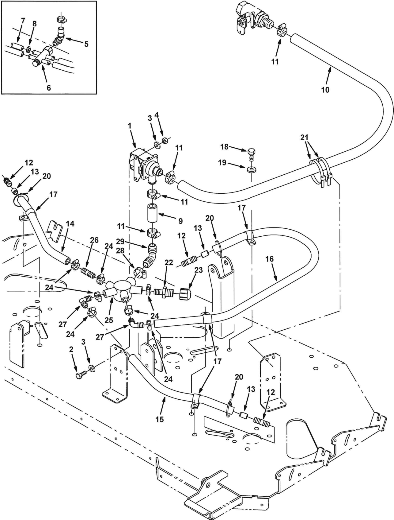
Fig. 21 - Max Pro 1200 (Disc-Brush) Solution Valve Group
