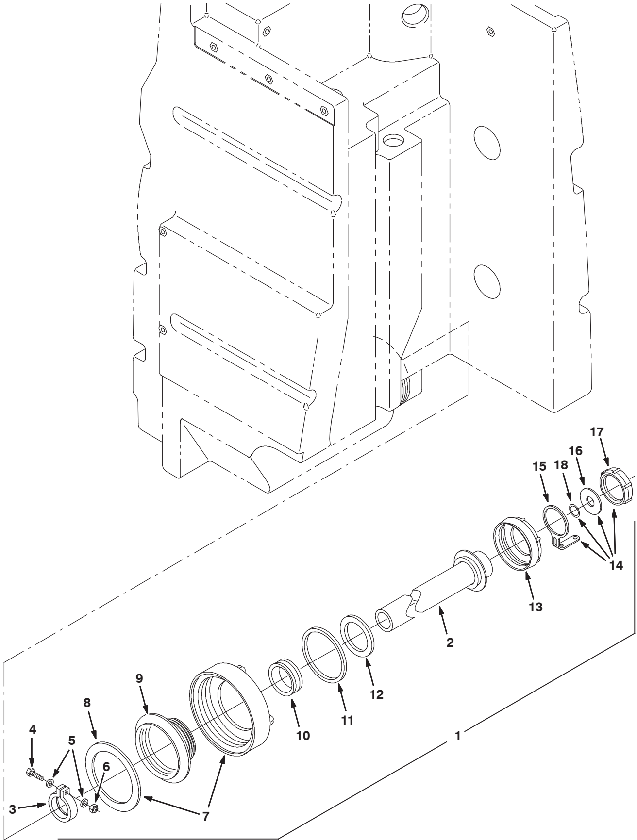
Fig. 24 - Recovery Tank Drain Assembly
