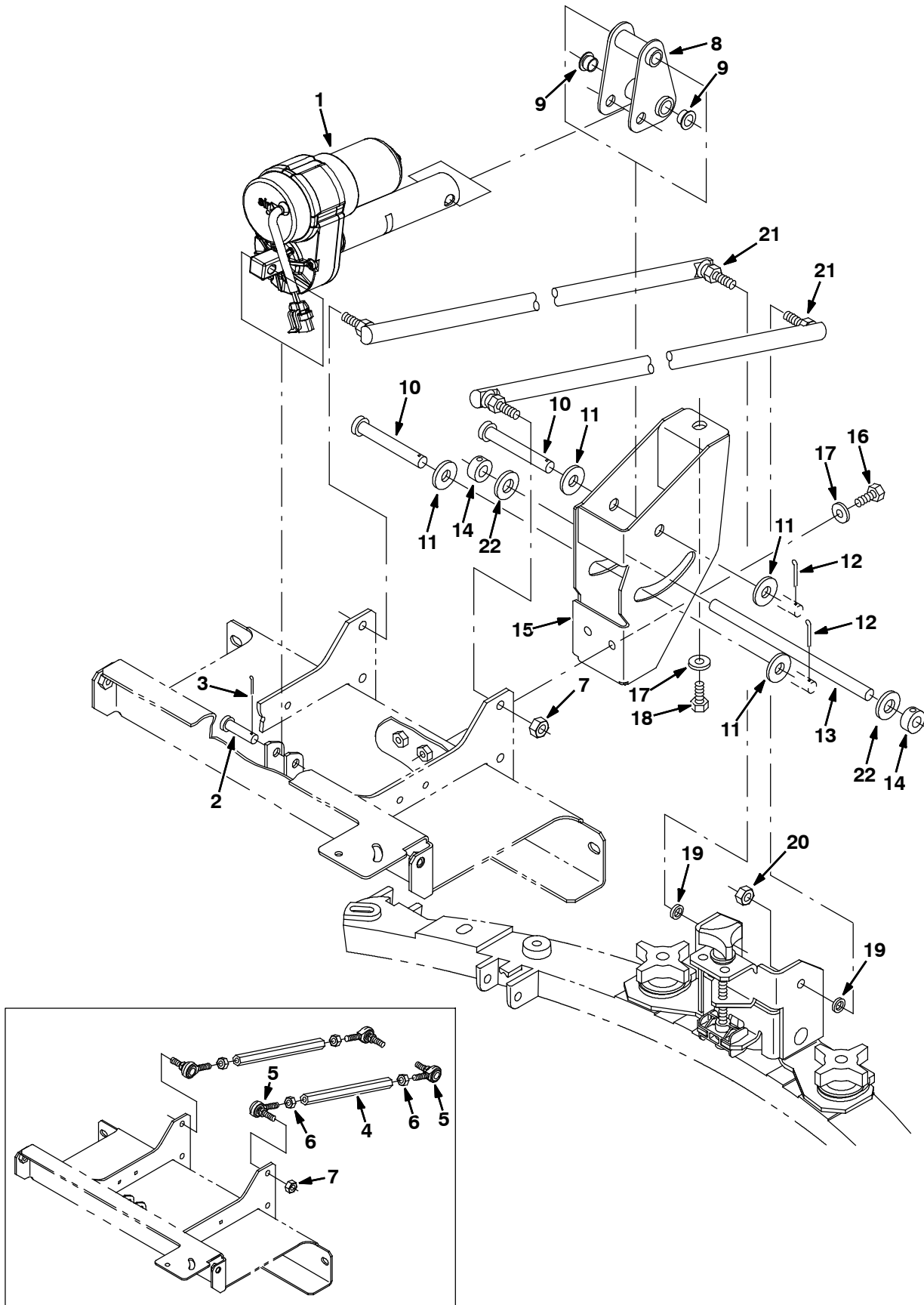
Fig. 49 - Rear Squeegee Lift Group
