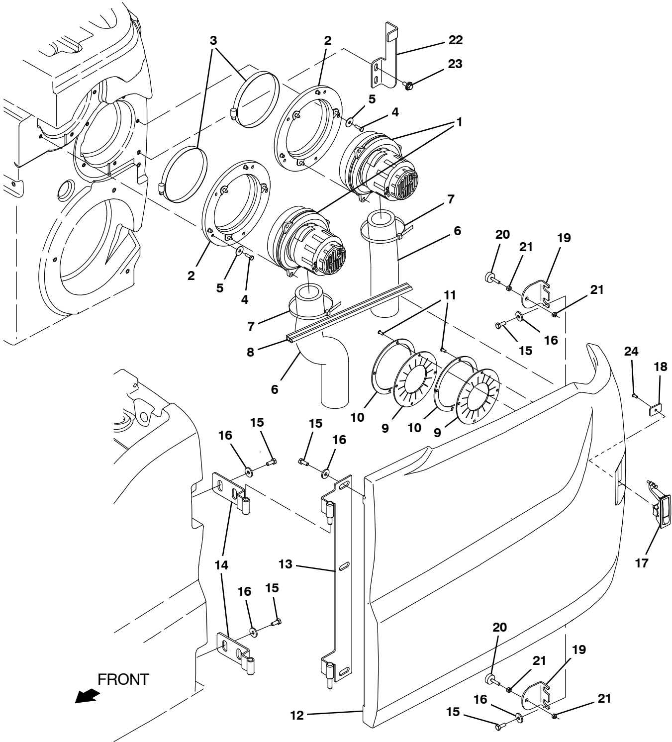
Fig. 25 – Vacuum Fans and Rear Side Door Group
