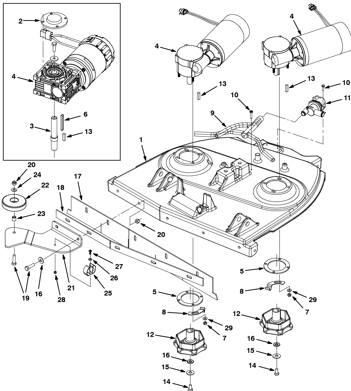
Fig. 16 - Disk Scrub Head Drive Motor Group, 650 mm
