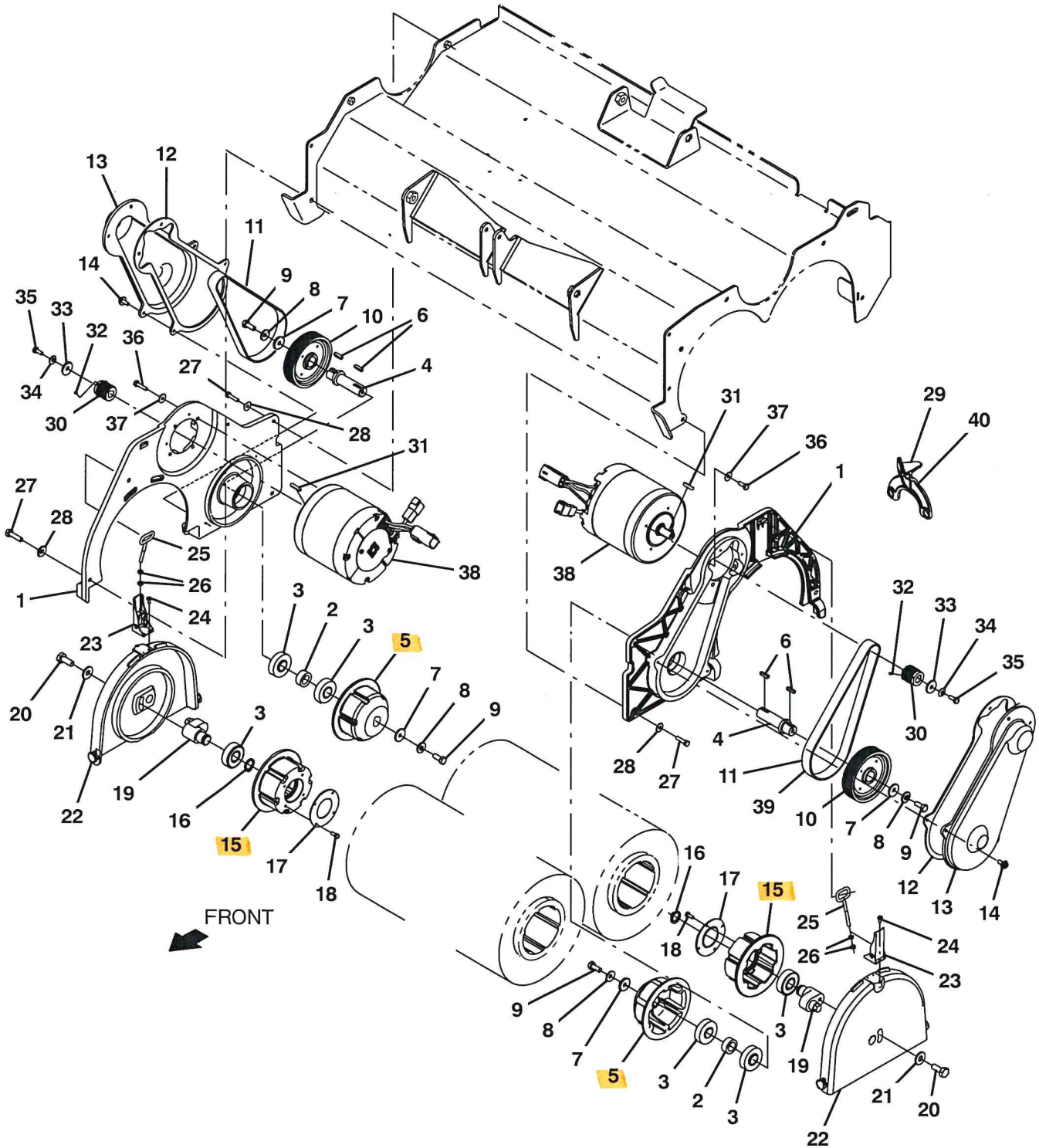
Fig. 26 – Scrub Head Drive Motors Group, Cylindrical
