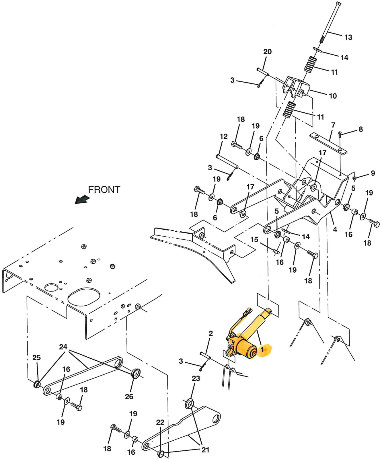
Fig. 15 - Scrub Head Lift Group
