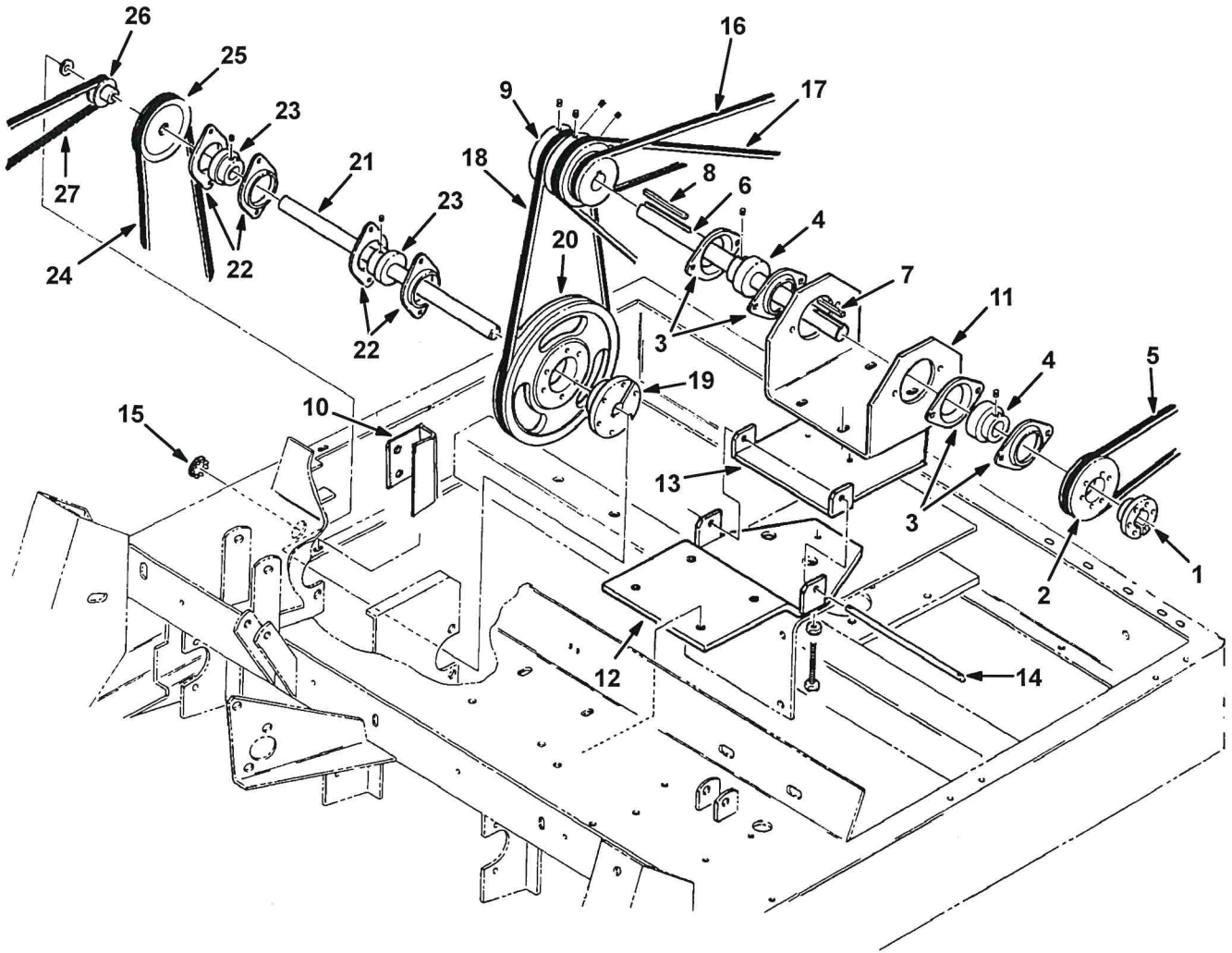
Fig. 17 - Drive System - Getriebe System - Transmission
