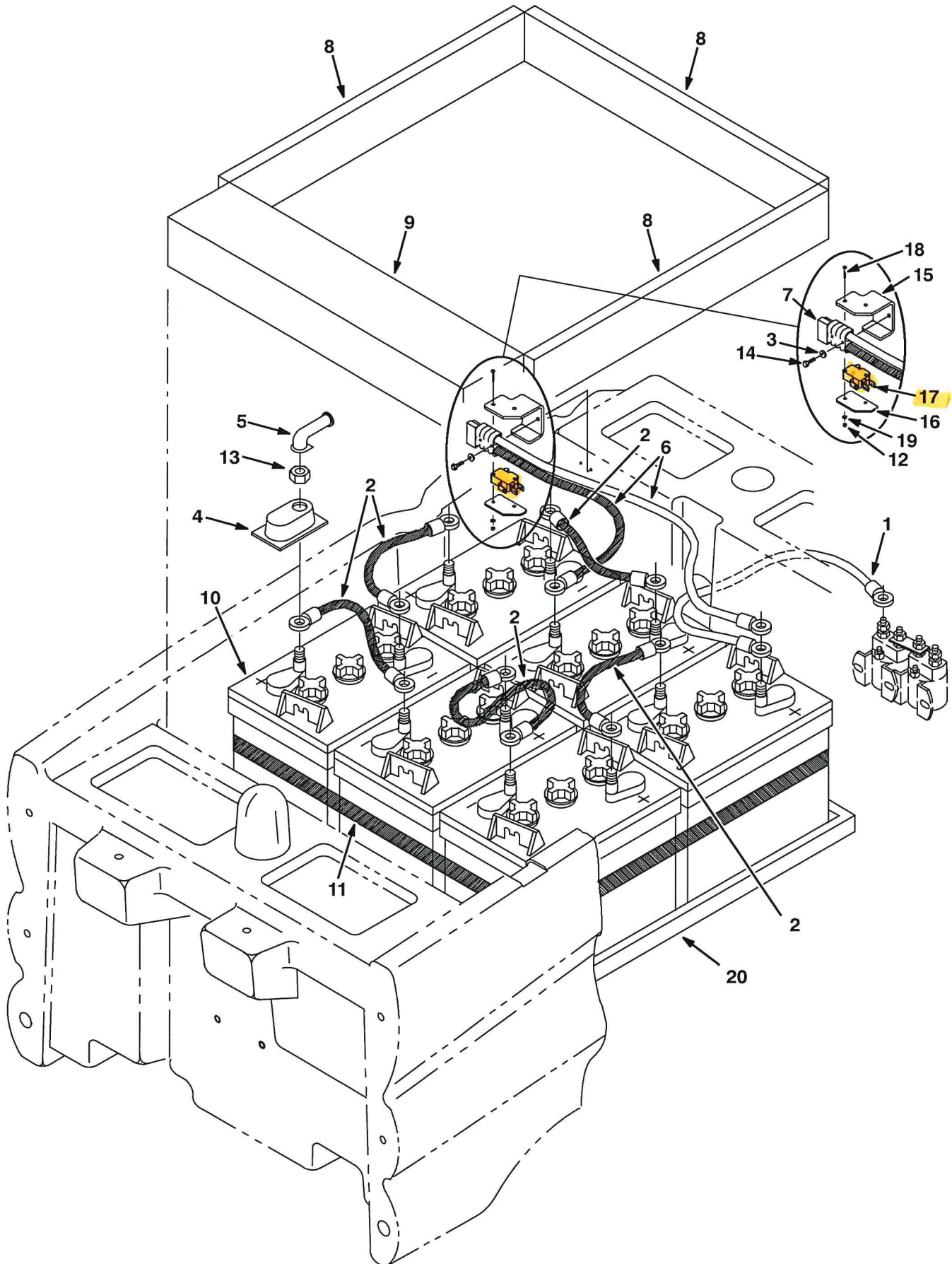
Fig. 16 - Battery Group
