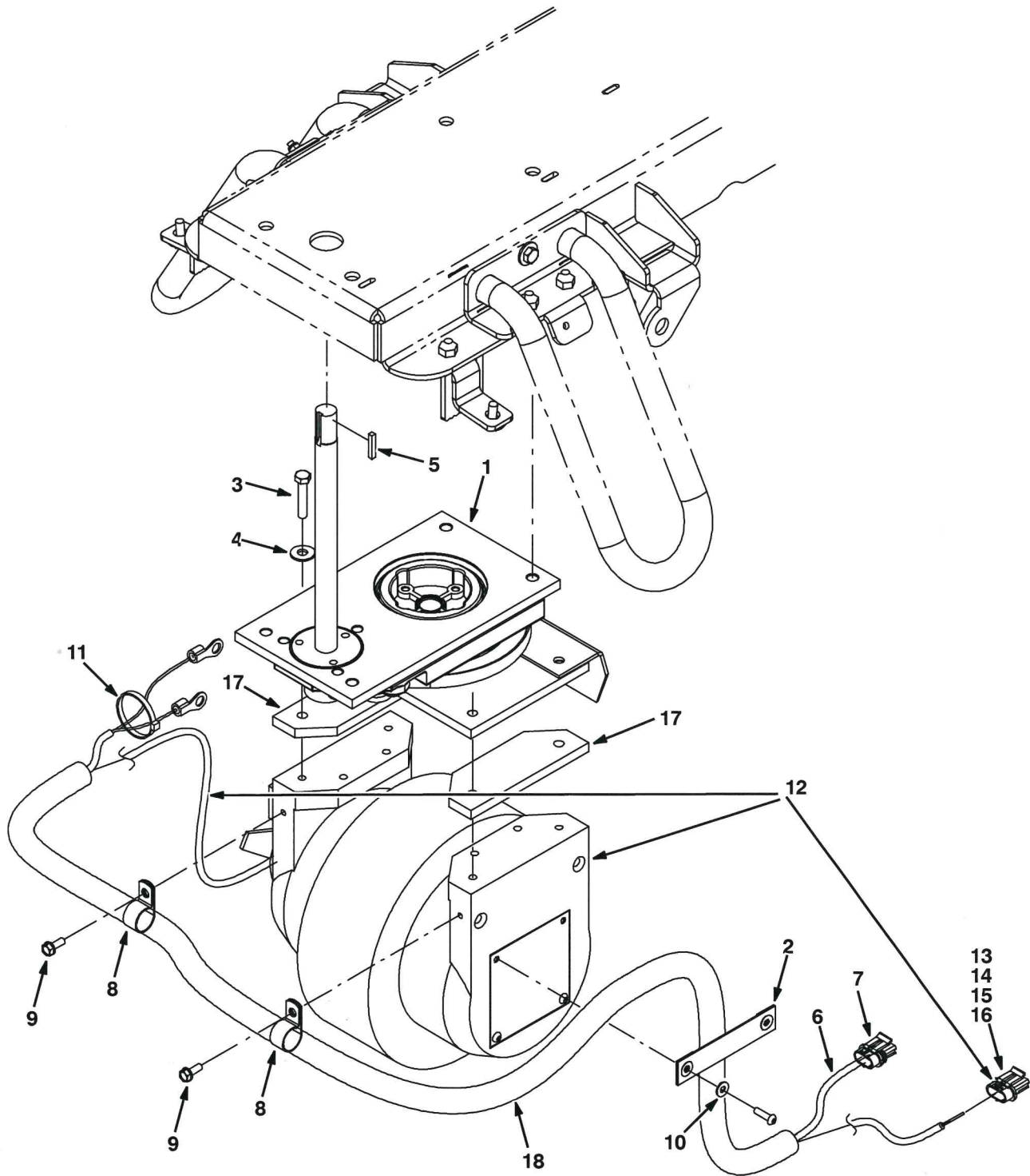
Fig. 11 - Front Drive Wheel Group (S/N 00000-05315)
