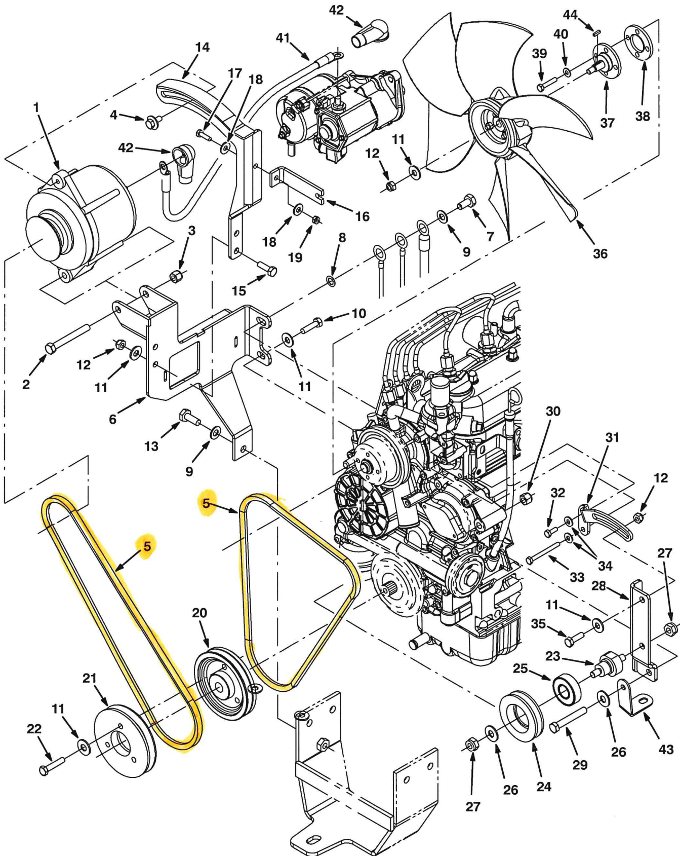
Fig. 14 - Engine Alternator Group, Diesel
